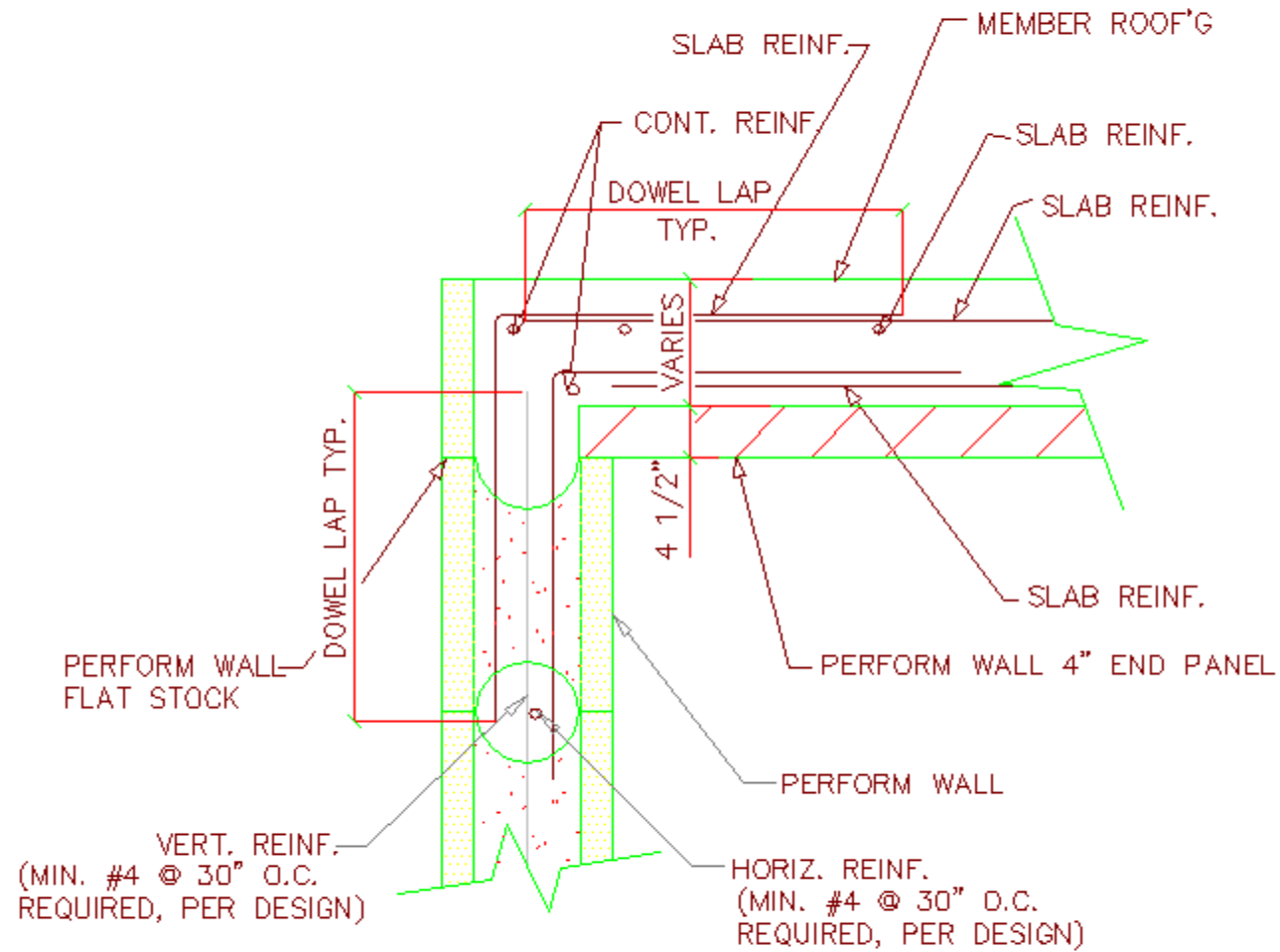
EXAMPLE OF SUPPORTING CONCRETE FLOOR OR ROOF
