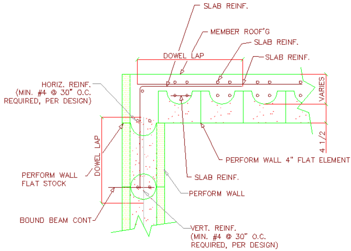
EXAMPLE OF SUPPORTING CONCRETE FLOOR OR ROOF USING END PANELS
