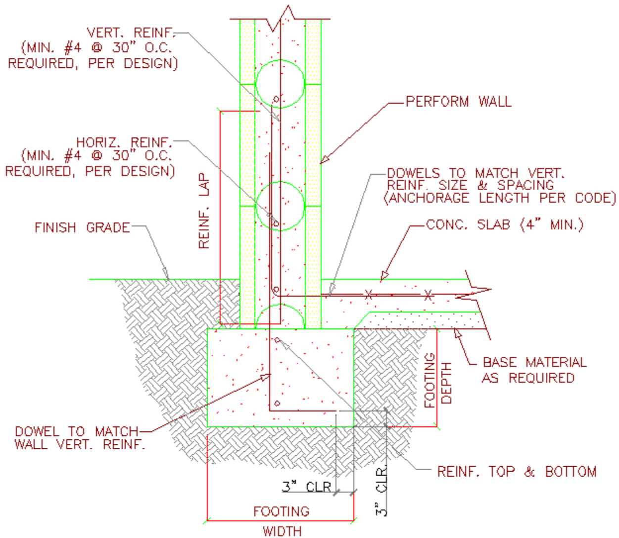
EXTERIOR WALL FOOTING WITH SLAB
