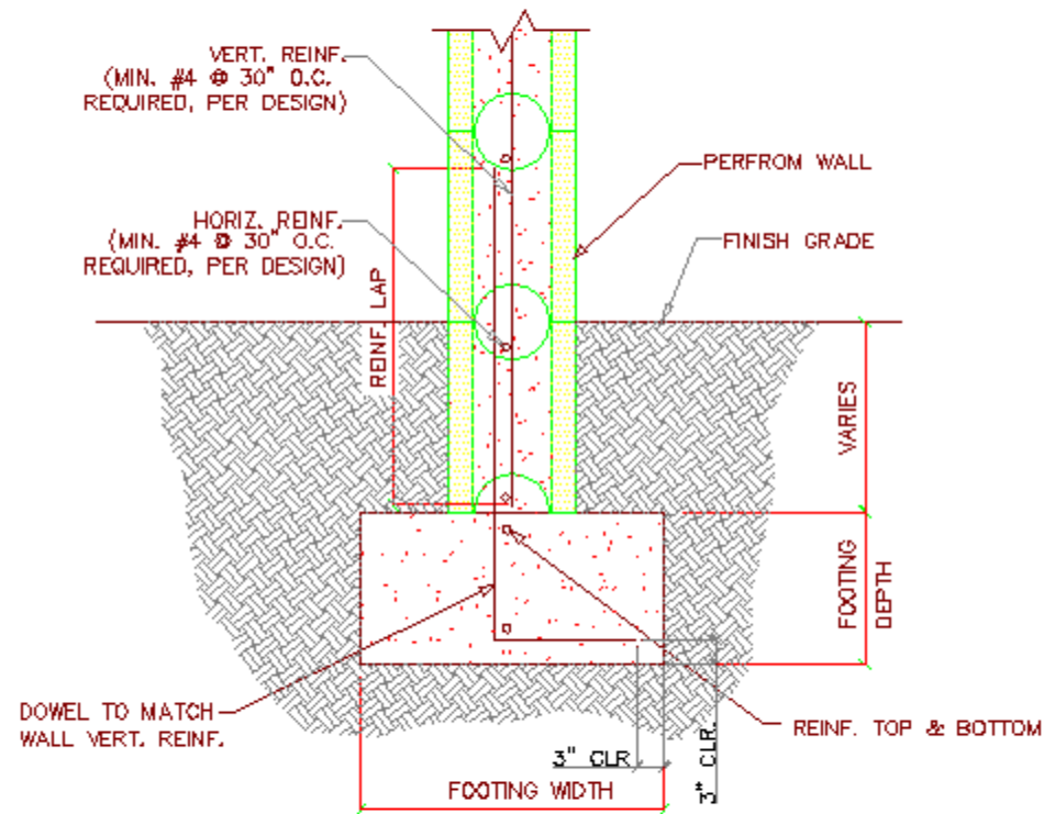
FOOTING WITHOUT SLAB
