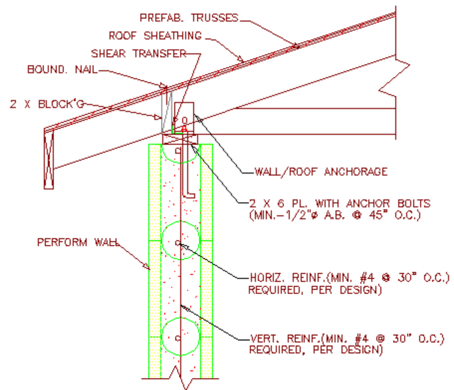
ROOF TRUSS WITH ANCHOR
