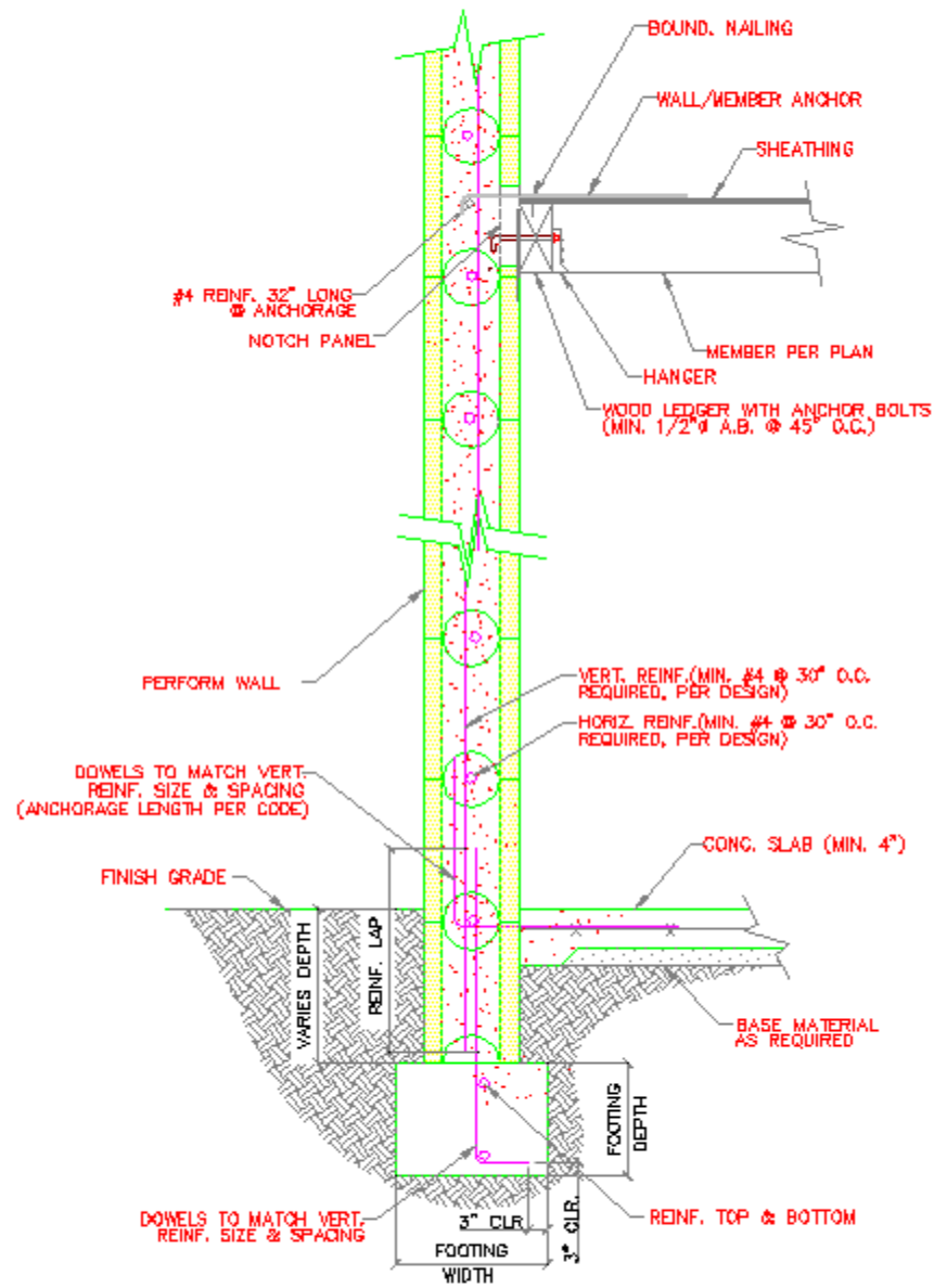
SECTION SUPPORTING FLAT FLOOR OR ROOF WITH PREFAB JOIST
