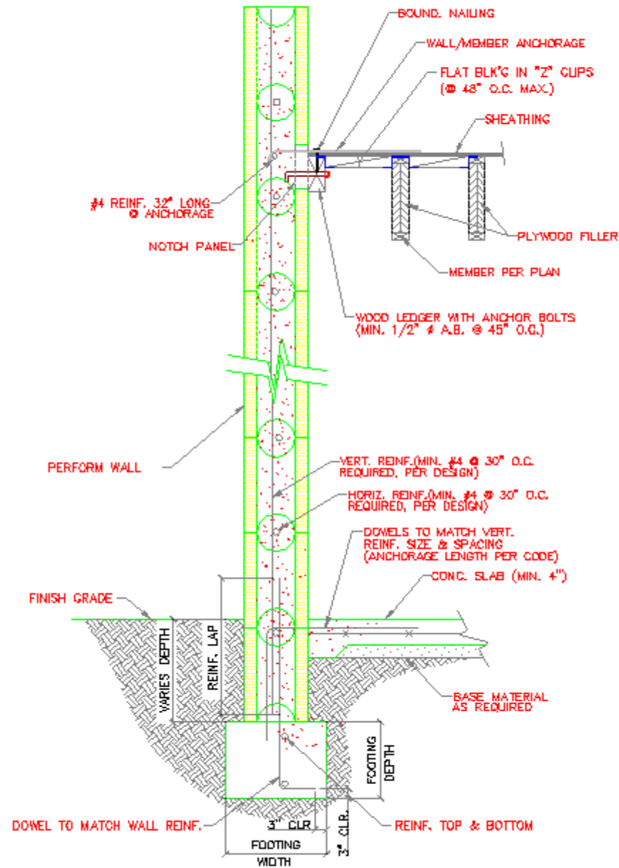
FLAT ROOF SECTION
