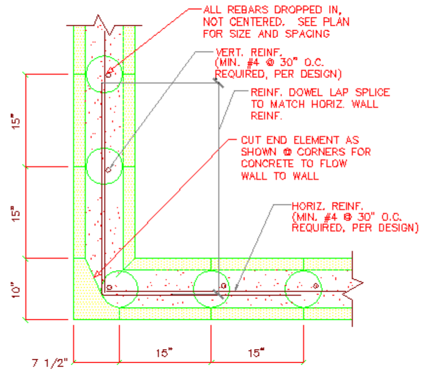
END PANEL CAPPED CORNER CONNECTION
